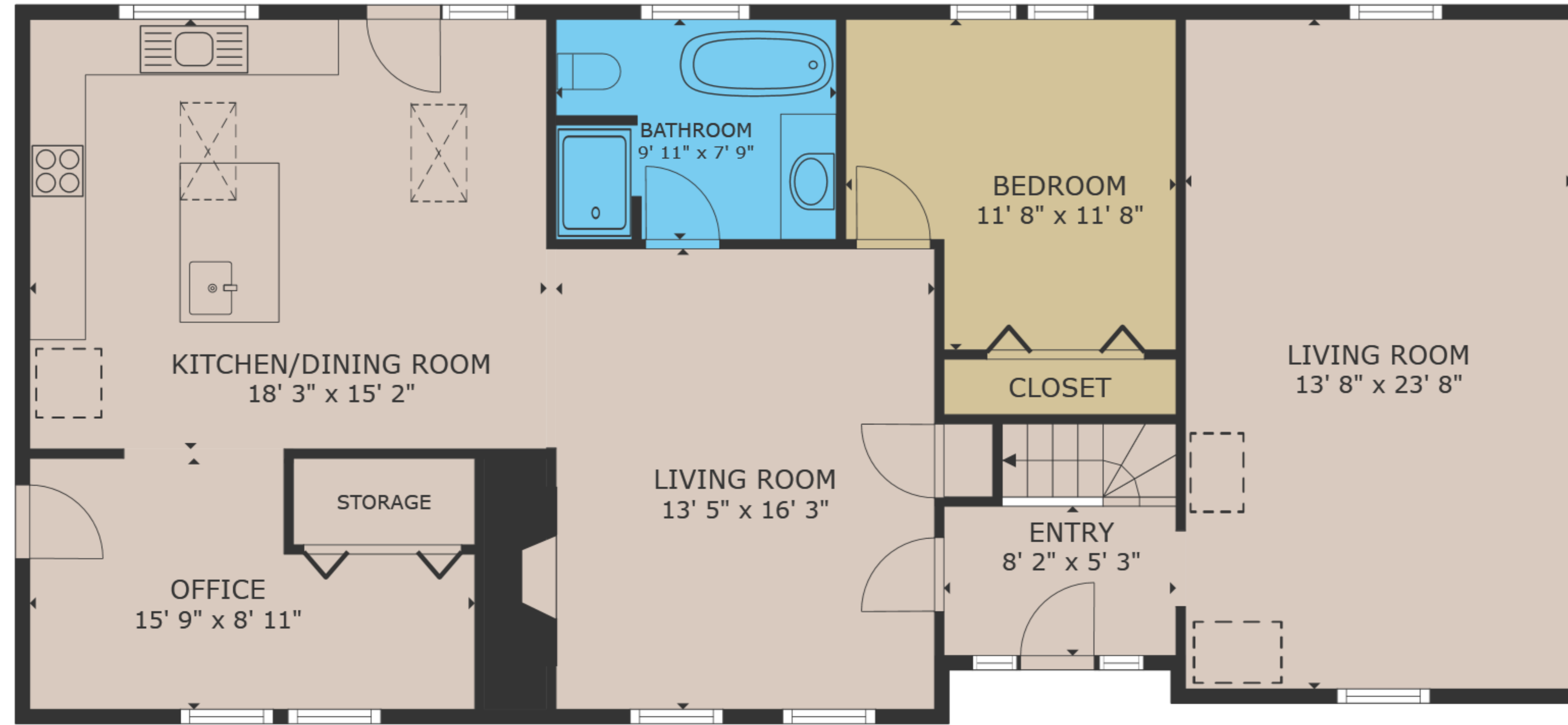
FLOOR 1
